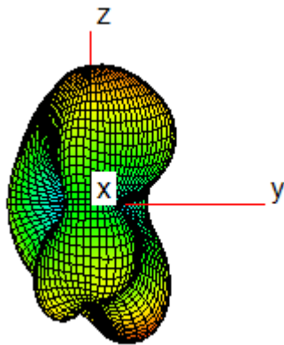
3D
