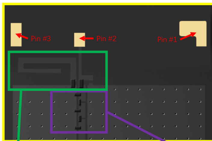
Antenna Tuning
