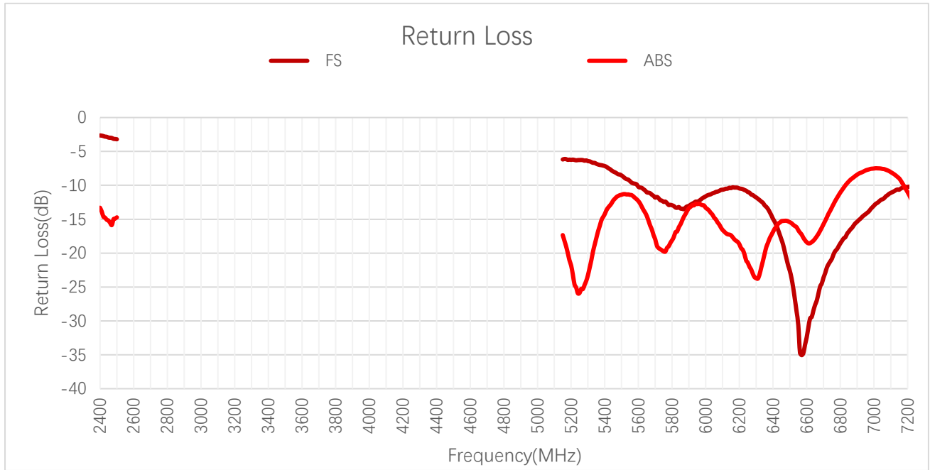
Return Loss
