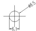
Recommended Mounting Hold
