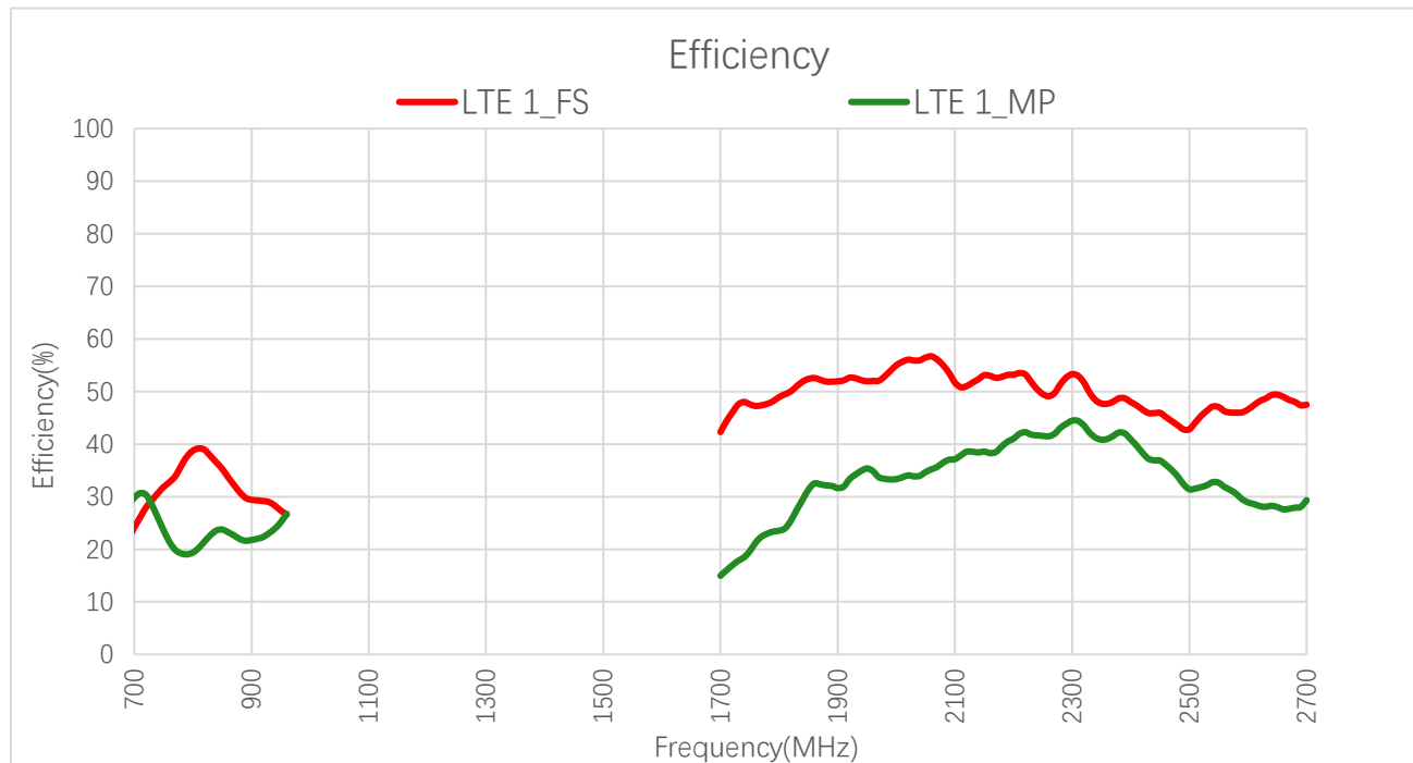
Efficiency (%) – LTE 1
