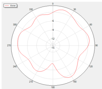
Phi=90 Freq=2450MHz
