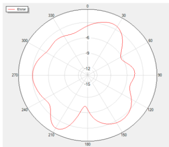
Phi=90 Freq=2140MHz
