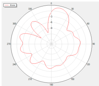
Theta=90 Freq=2450MHz
