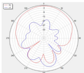
Phi=0 freq=1602MHz
