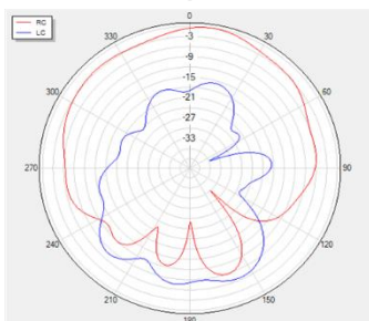
Phi=90 freq=1575MHz
