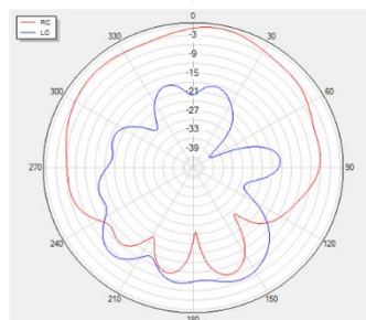
Phi=90 freq=1602MHz
