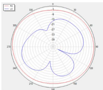
Theta=90 freq=1575MHz
