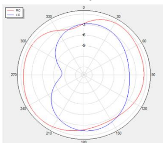
Theta=90 freq=1176MHz
