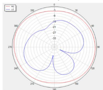
Theta=90 freq=1561MHz
