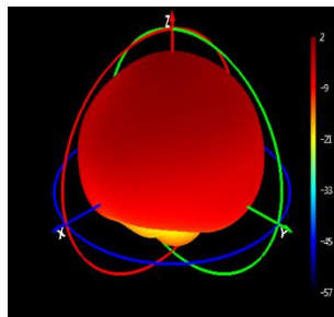
Phi=0 freq=1575MHz
