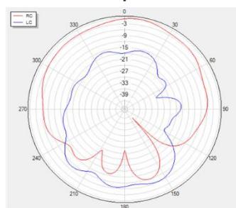
Phi=90 freq=1561MHz
