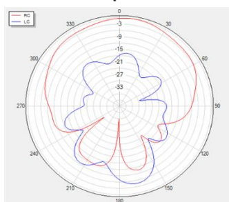
Phi=0 freq=1561MHz
