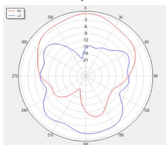
Phi=0 freq=1176MHz
