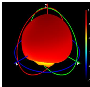
Phi=0 freq=1602MHz
