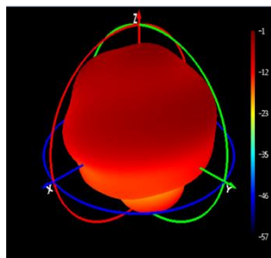
Phi=0 freq=1176MHz
