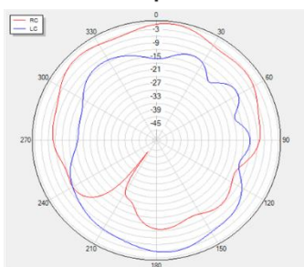
Phi=90 freq=1176MHz
