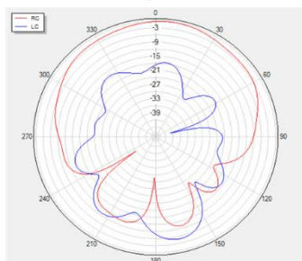
Phi=0 freq=1575MHz
