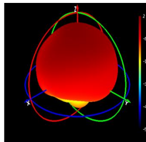
Phi=0 freq=1561MHz
