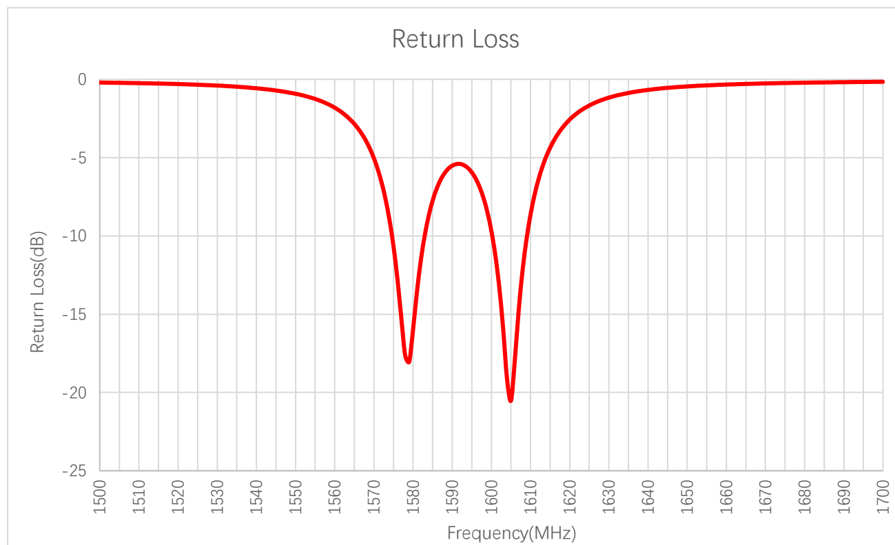
Return Loss (dB)
