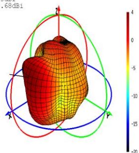
Phi=0 Freq=2450MHz
