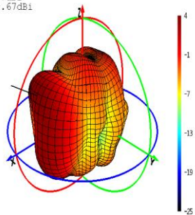
Phi=0 Freq=2140MHz
