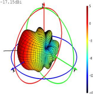
Phi=0 Freq=2350MHz
