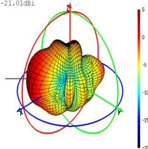
Phi=0 Freq=2600MHz
