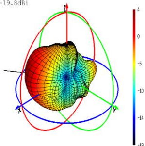
Phi=0 Freq=2450MHz
