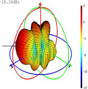
Phi=0 Freq=2140MHz
