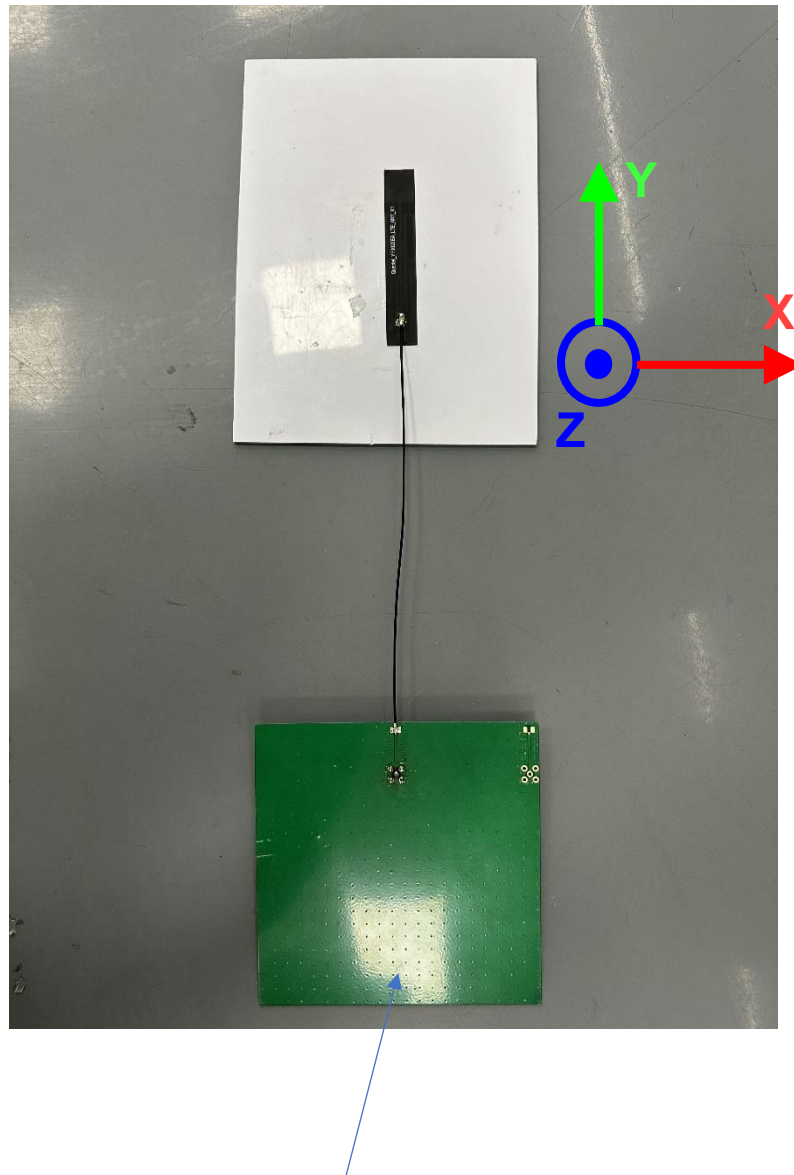
130 × 130 mm EVB
