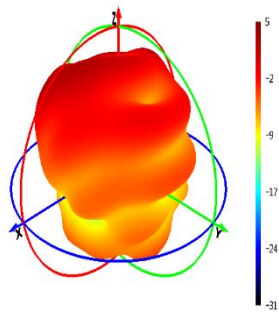
4000 MHz
