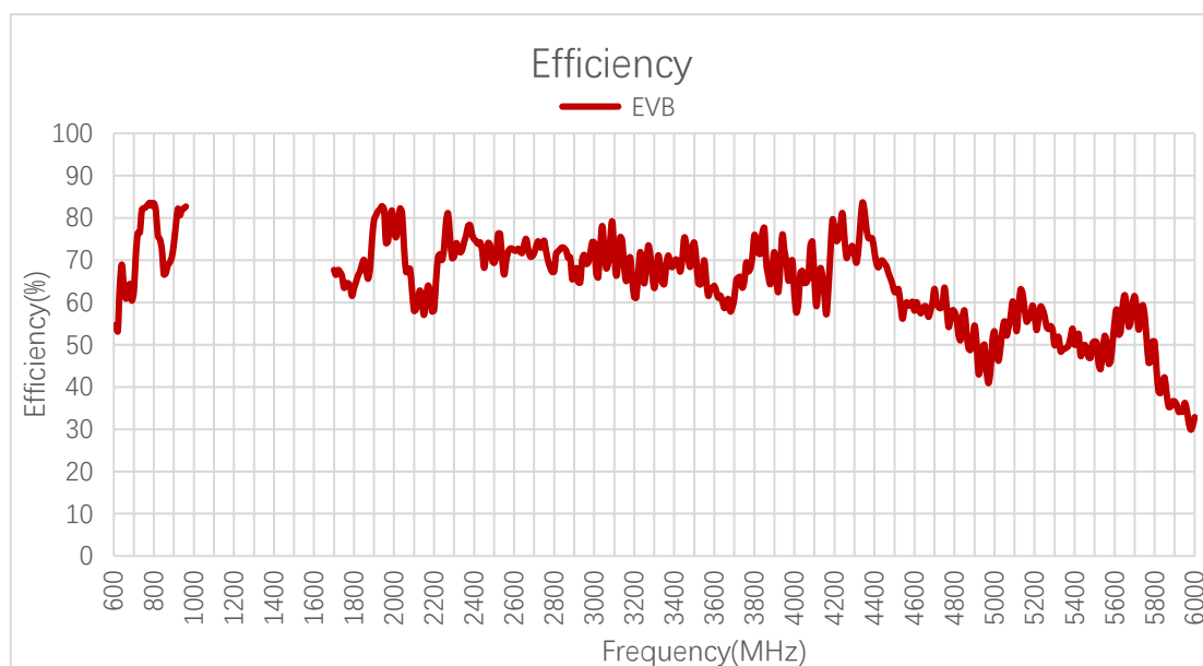
Efficiency (%)
