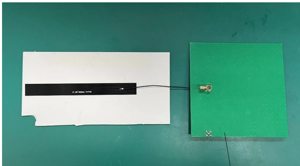
130 × 130 mm EVB
