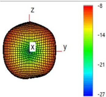
420 MHz
