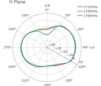
H Plane
