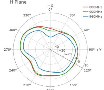
H Plane
