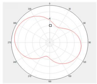
Theta=90 Freq=1602MHz
