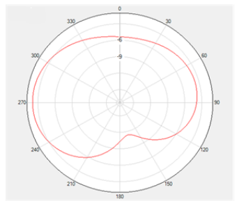
Theta=90 Freq=1176MHz
