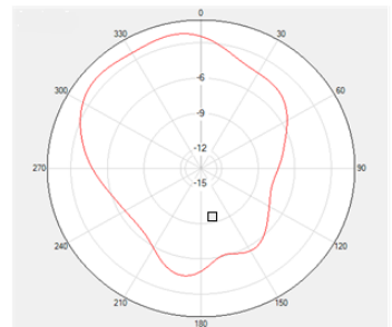
Phi=90 Freq=157.5MHz
