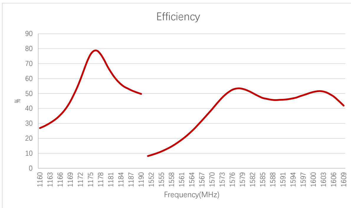
Efficiency (%) - GNSS
