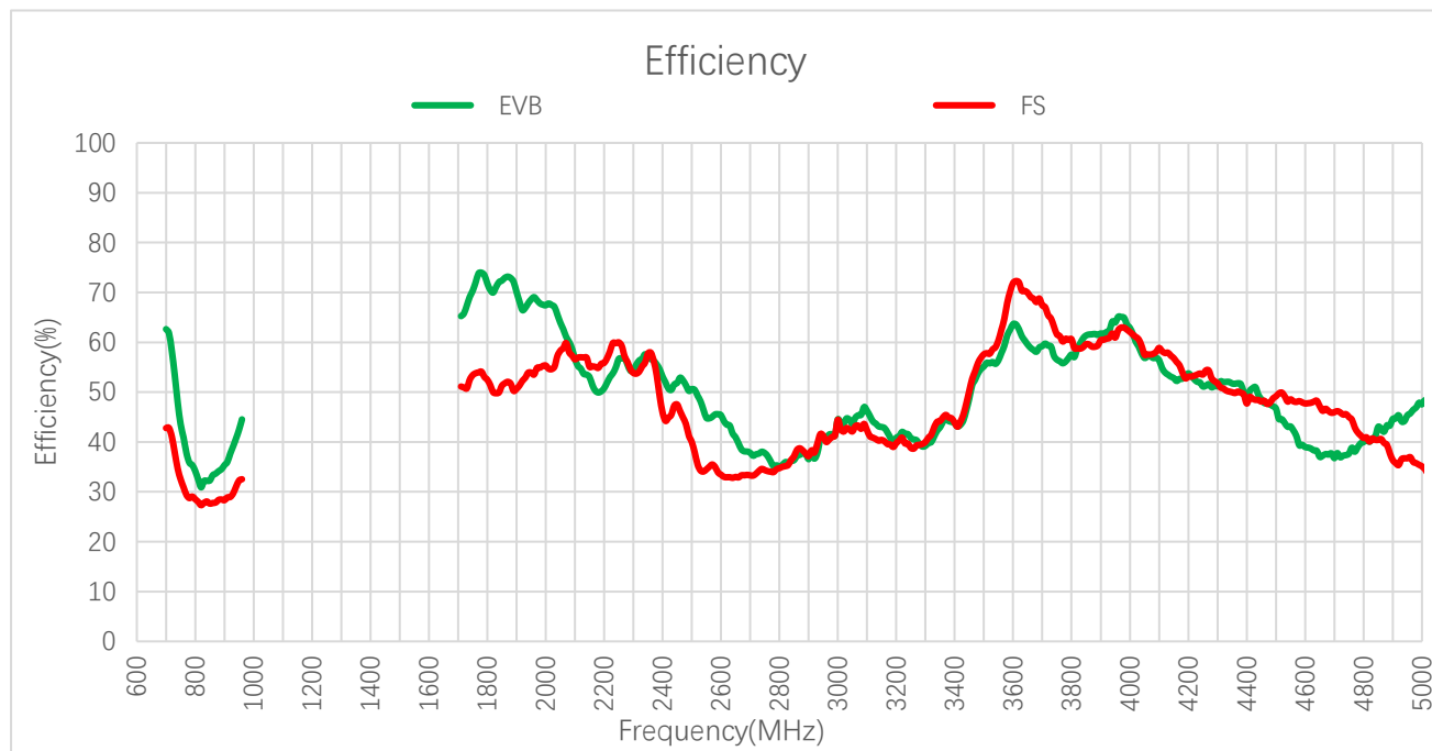
Efficiency (%)
