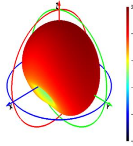
1561 MHz
