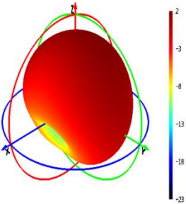
1575 MHz
