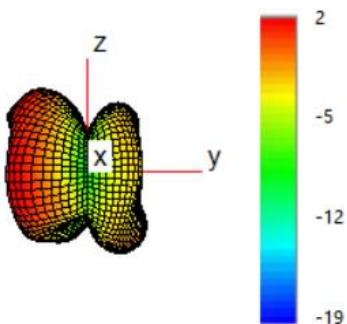
1880 MHz
