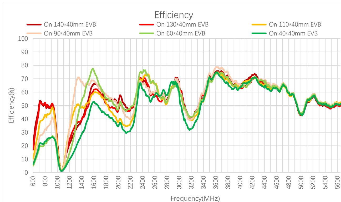
Efficiency (%)
