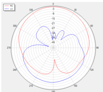
Phi=0 freq=1575MHz
