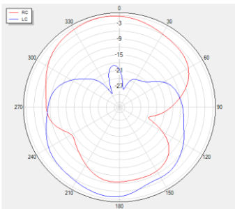
Phi=90 freq=1176MHz
