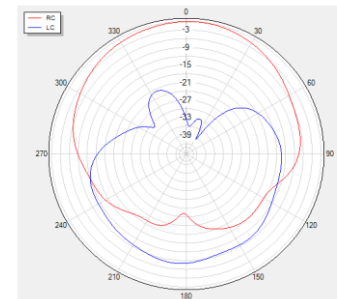
Phi=90 freq=1602MHz
