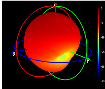
Phi=90 freq=1176MHz
