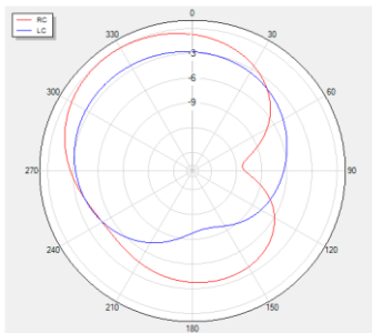
Theta=90 freq=1176MHz
