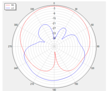
Phi=0 freq=1561MHz
