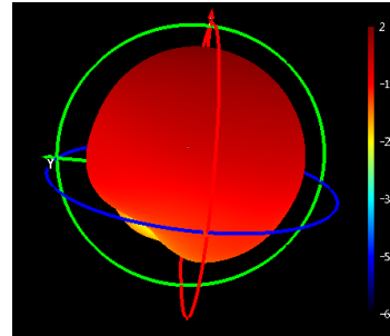
Phi=90 freq=1602MHz
