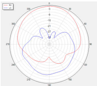
Phi=90 freq=1575MHz
