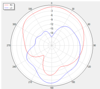
Phi=0 freq=1176MHz
