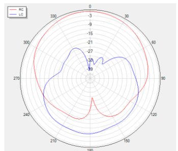
Phi=0 freq=1602MHz
