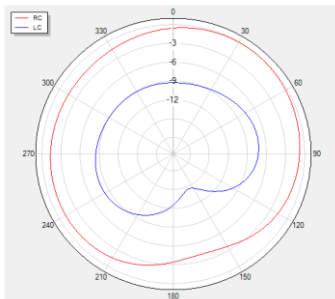
Theta=90 freq=1575MHz
