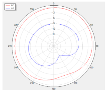
Theta=90 freq=1561MHz
