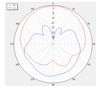
Phi=90 freq=1561MHz
