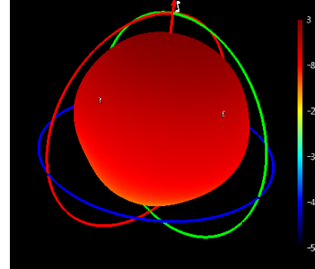
Phi=90 freq=1561MHz
