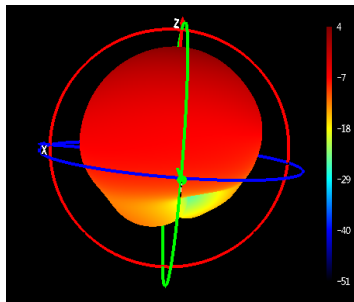
Phi=90 freq=1575MHz
