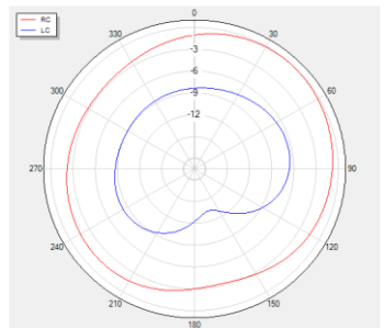
Theta=90 freq=1602MHz
