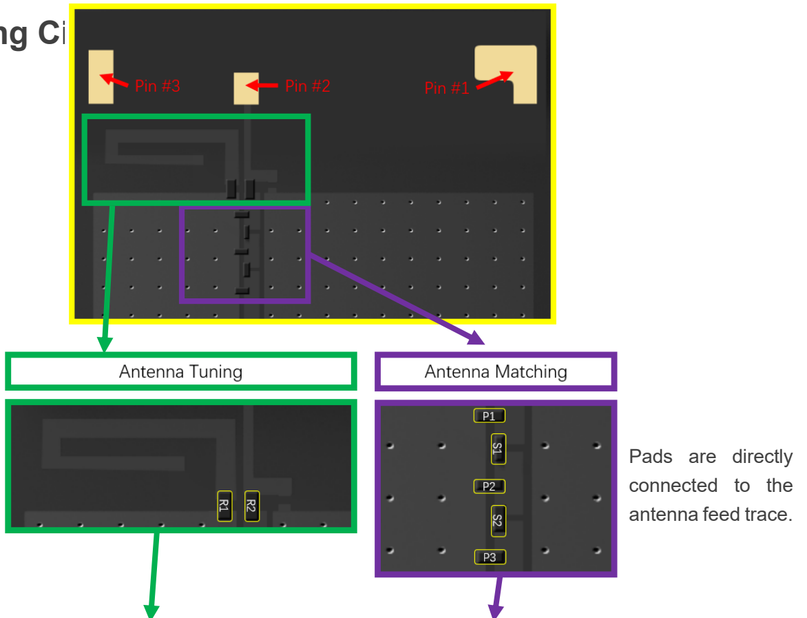
Demo Board Top View
