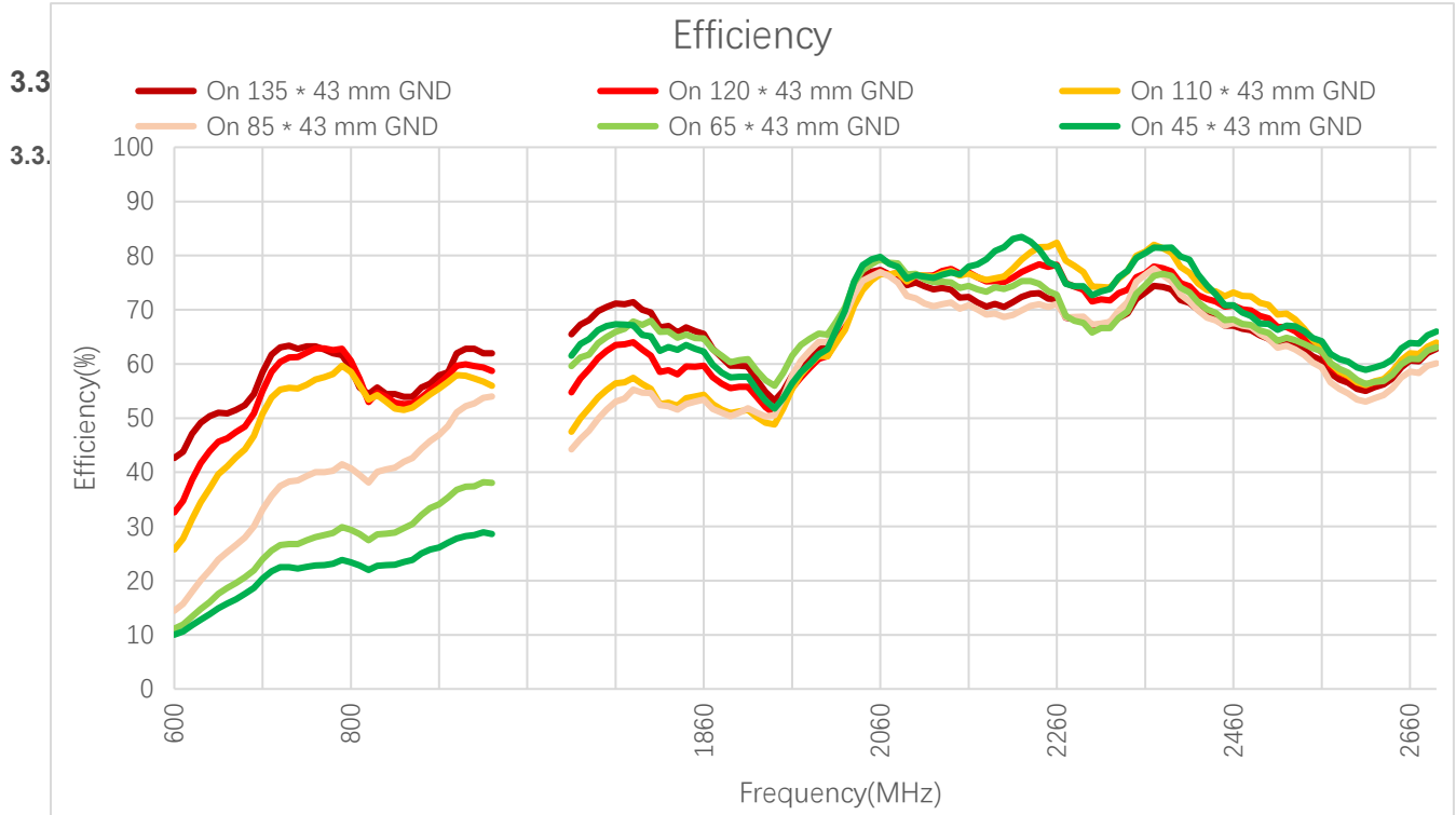
Efficiency (%)
