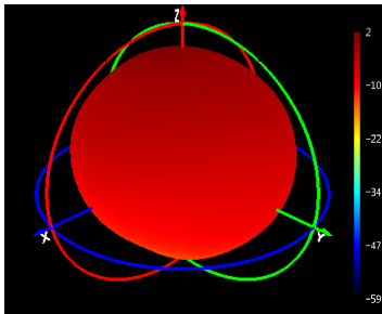
Phi=90 freq=1575MHz
