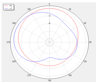
Theta=90 freq=1176MHz
