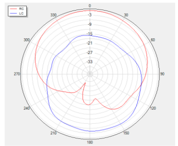
Phi=0 freq=1561MHz
