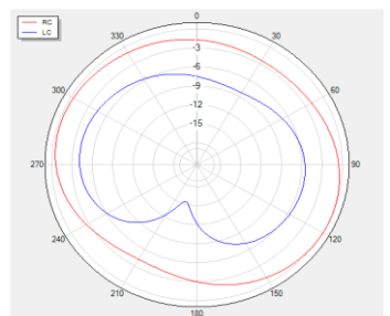
Theta=90 freq=1602MHz
