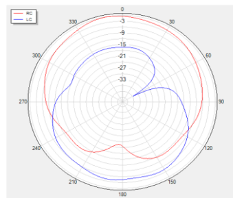
Phi=90 freq=1561MHz
