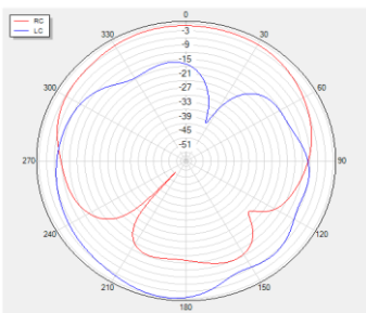
Phi=90 freq=1176MHz
