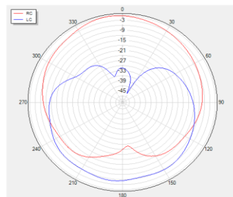
Phi=90 freq=1602MHz
