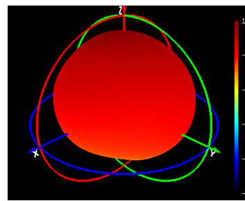
Phi=90 freq=1602MHz
