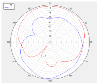
Phi=0 freq=1176MHz
