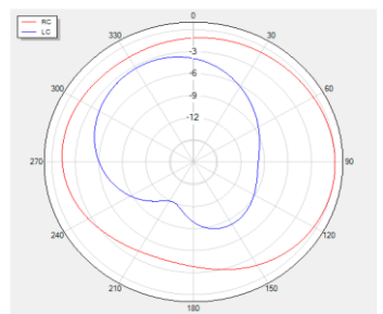
Theta=90 freq=1561MHz
