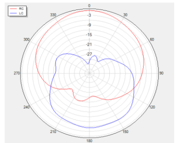
Phi=0 freq=1602MHz
