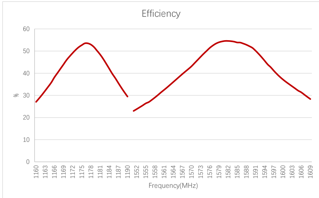
Efficiency (%)
