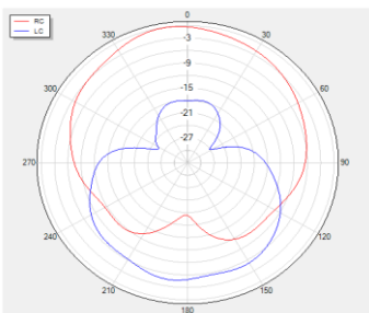
Phi=90 freq=1575MHz
