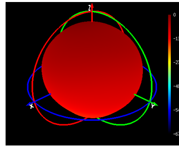
Phi=90 freq=1561MHz
