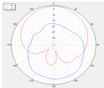
Phi=0 freq=1575MHz
