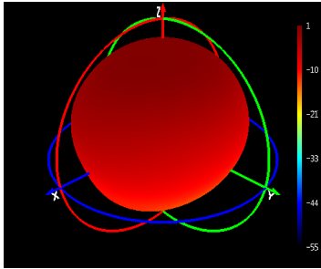
Phi=90 freq=1176MHz
