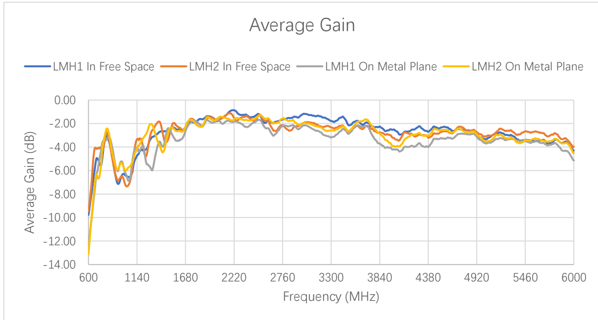
Average Gain (dB) – LMHs
