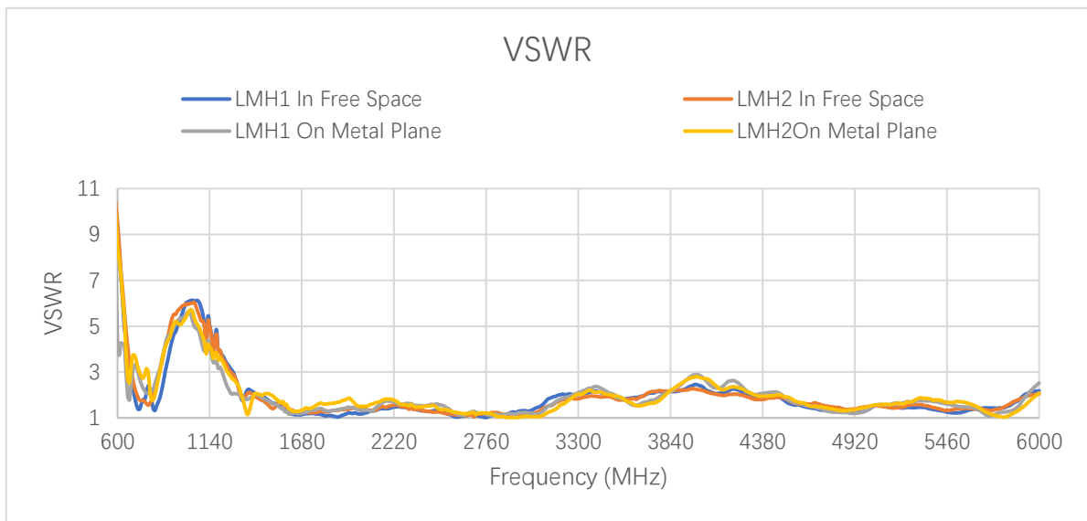
VSWR – LMHs
