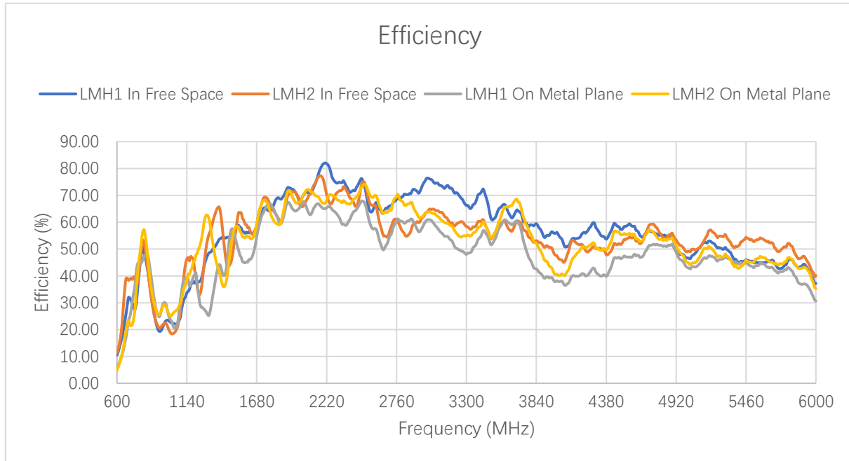
Efficiency (%) – LMHs
