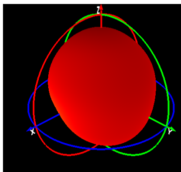
Phi=90 freq=1602MHz
