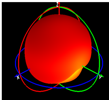
Phi=90 freq=1561MHz
