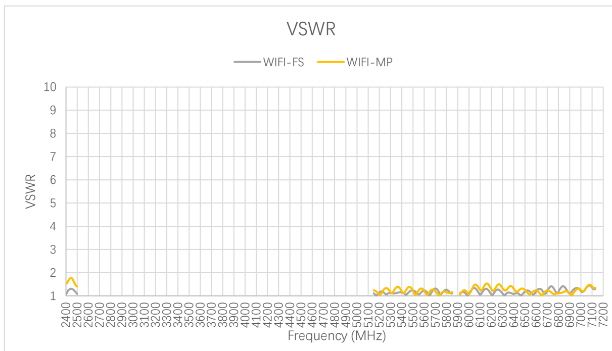
VSWR – Wi-Fi
