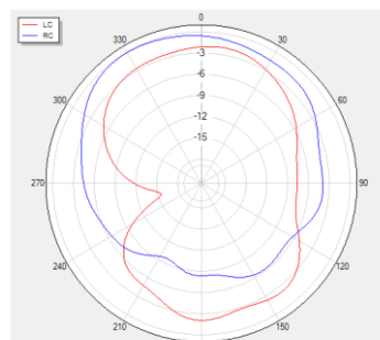
Phi=0 freq=1575MHz
