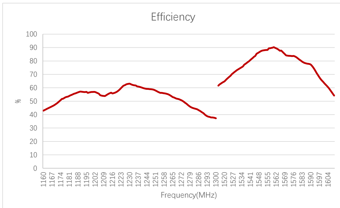
Efficiency (%)
